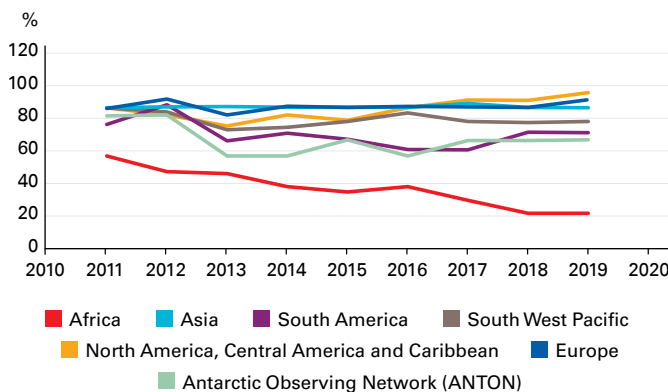
Figure 14: Percentage of dedicated upper-air stations reporting according to GRUAN requirements for the different WMO regions (2011-2019).
